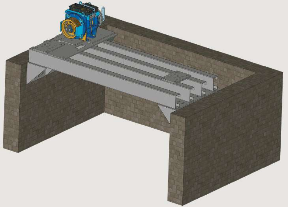
makine sehpaşı MRL DiSLiSiZ TiP 3 MR GEARLESS TYPE 3
